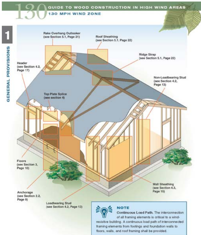
Figure 1. Master Building Frame
