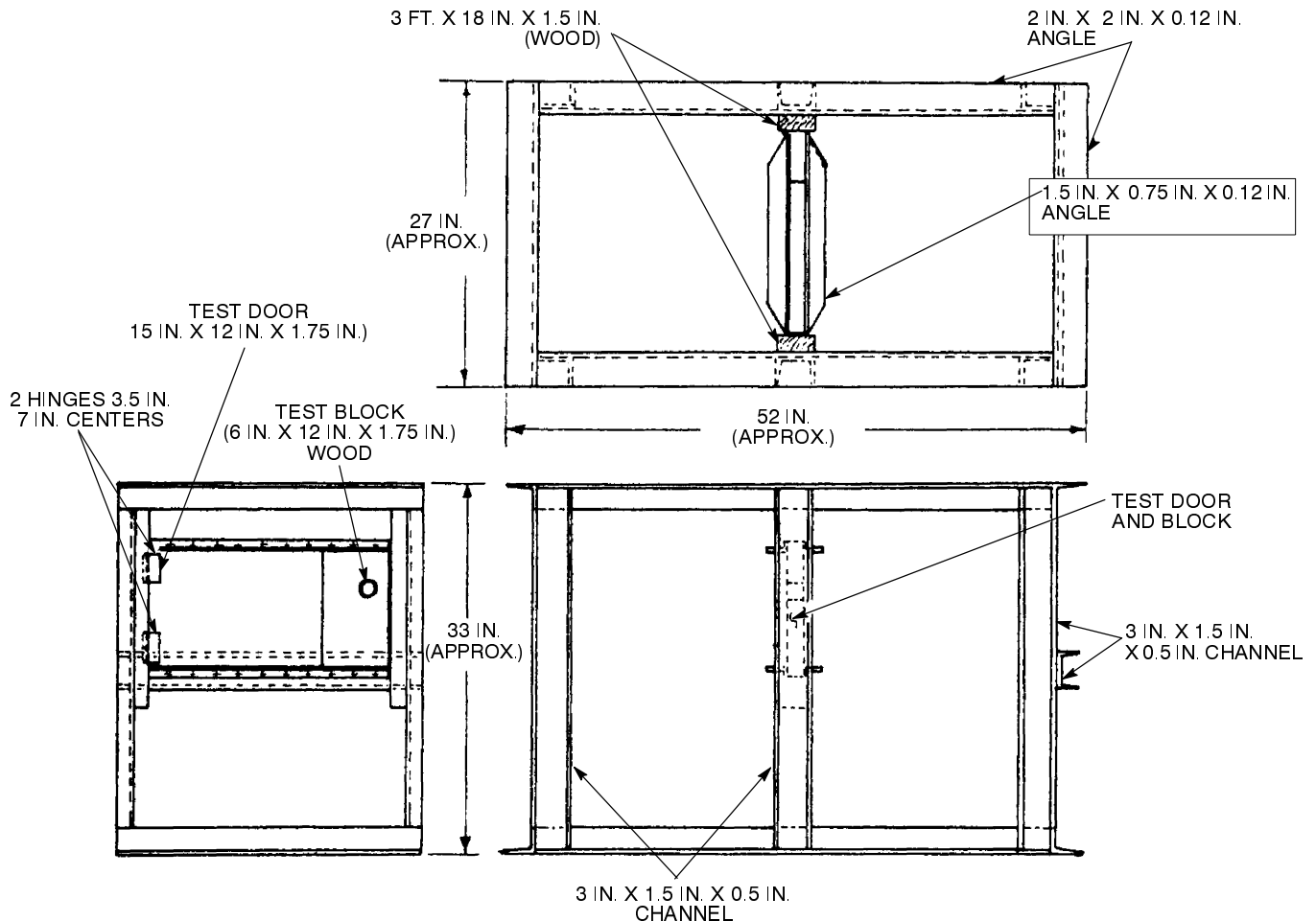
FIGURE 12-10-2-1—STATIC LOADING FIXTURE
