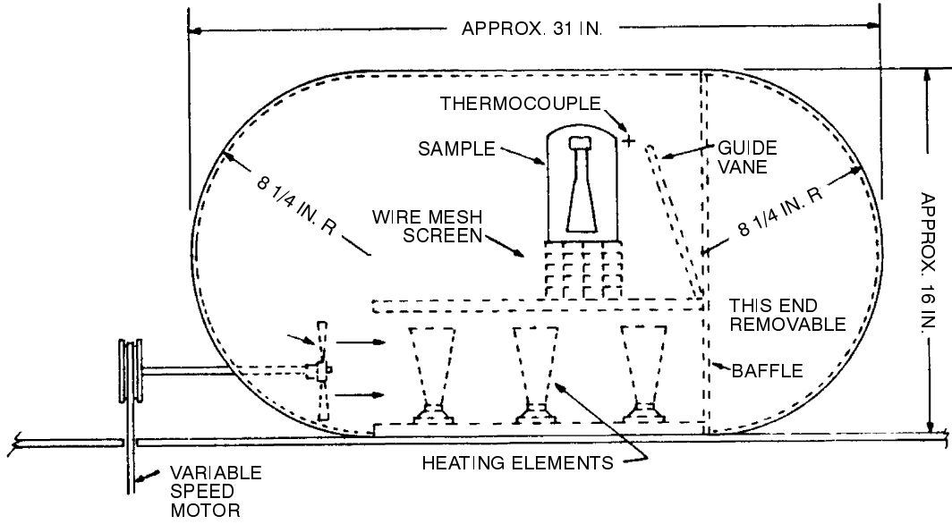
FIGURE 12-72-2-3—TEST OVEN
