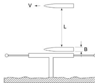
FIGURE 31F-5-4—PASSING VESSEL
