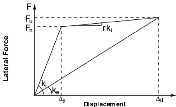
FIGURE 31F-4-5—EFFECTIVE STIFFNESS, k_e [4.1]
