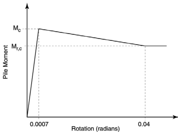
FIGURE 31F-7-12—JOINT ROTATION
