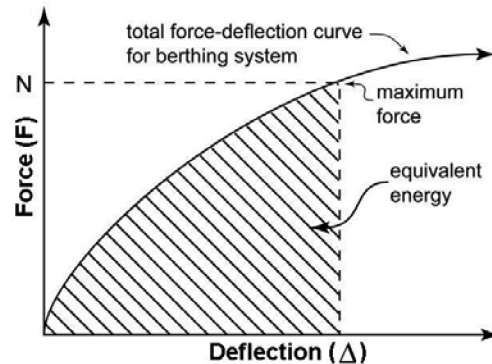
FIGURE 31F-5-5—BERTHING ENERGY CAPACITY
