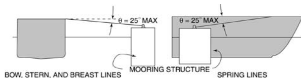
FIGURE 31F-5-3—VERTICAL LINE ANGLES [5.4]
