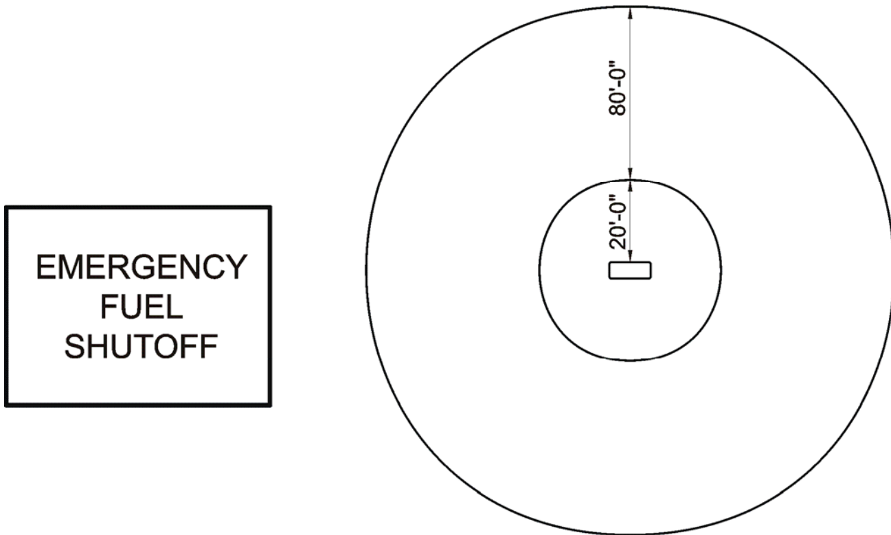
FIGURE 2303.2 EMERGENCY DISCONNECT SWITCH
