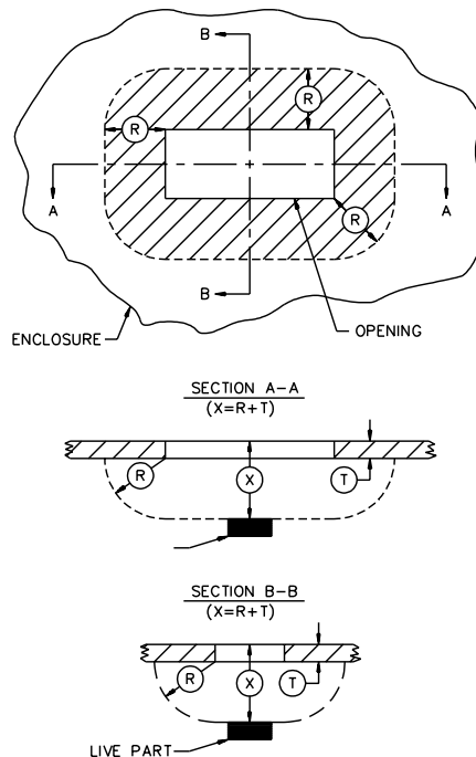
Figure 28.2 Opening in enclosure
