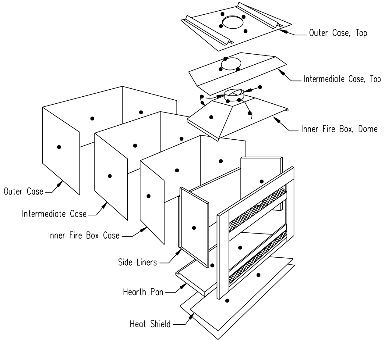
Figure 10.8 Typical thermocouple locations (Fire chamber assembly)
