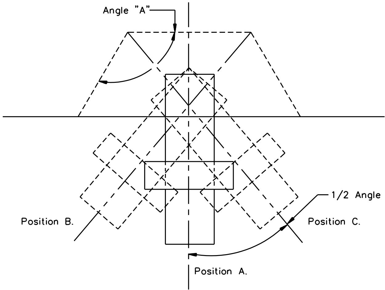
Figure 16.4 Inclined plane in position for strength test of back and side walls
