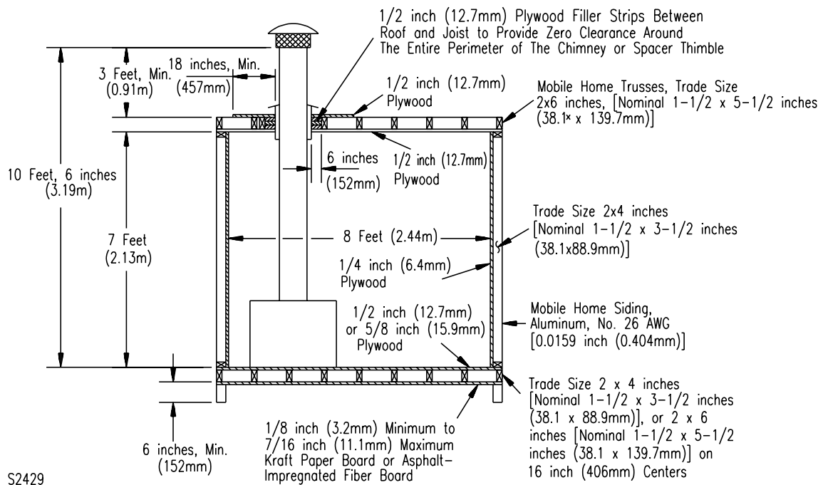
Figure 26.1 Manufactured home test enclosure
