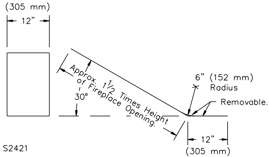
Figure 16.1 Inclined plane for strength test
