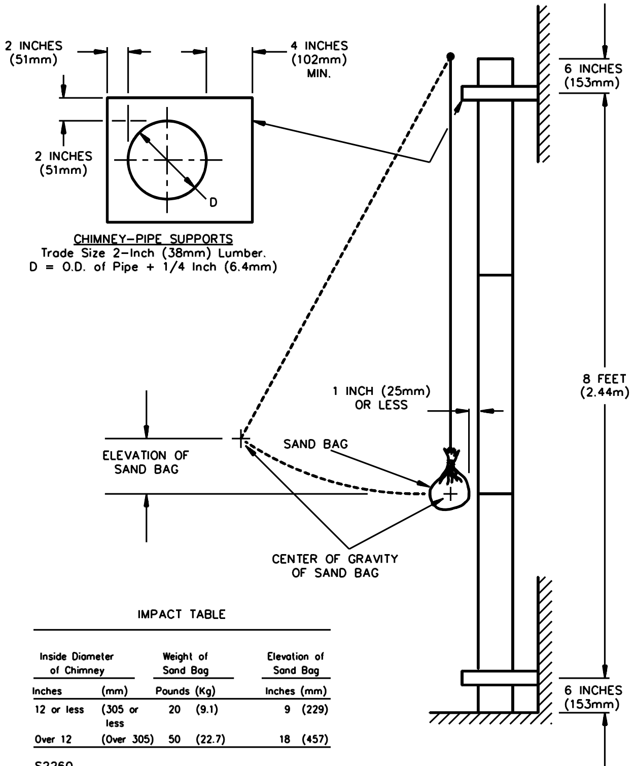
Figure 17.1 Strength test
