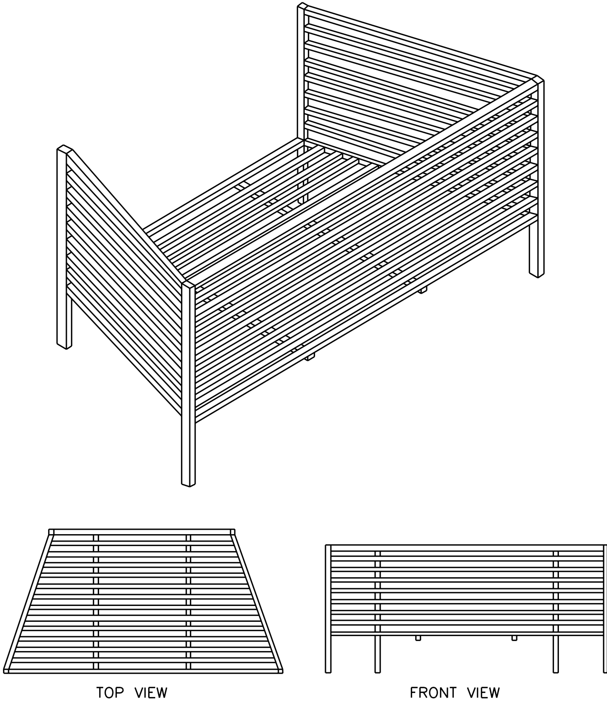
Figure 12.1 General form of charcoal basket
