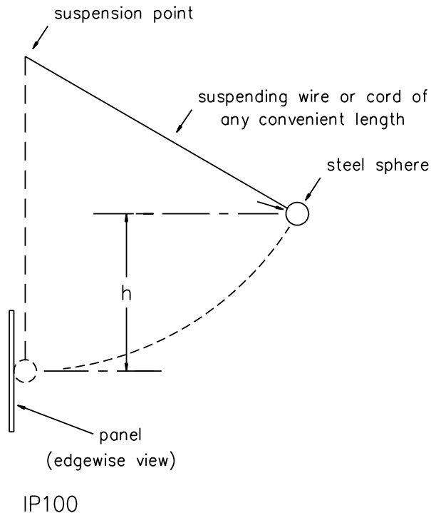
Figure 25.1 Impact test
