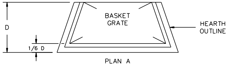
Figure 12.2 Typical relation of grate to hearth
