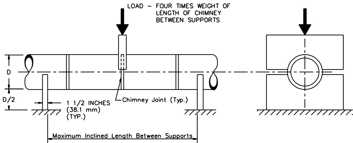
Figure 17.3 Chimney joint load test load
