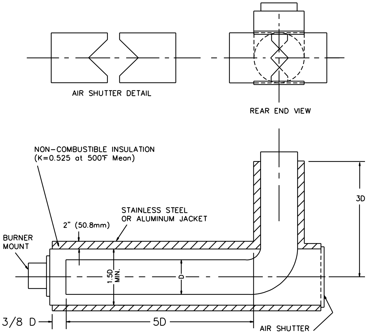
Figure 11.1 Flue-gas generator
