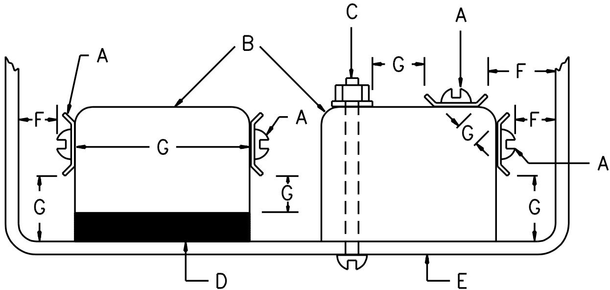
Figure 41.1 Component spacings
