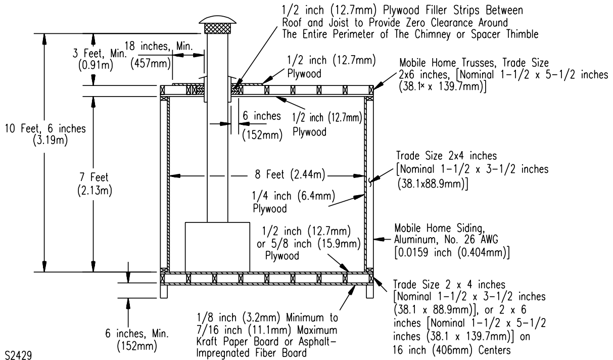
Figure 26.1 Mobile home test enclosure
