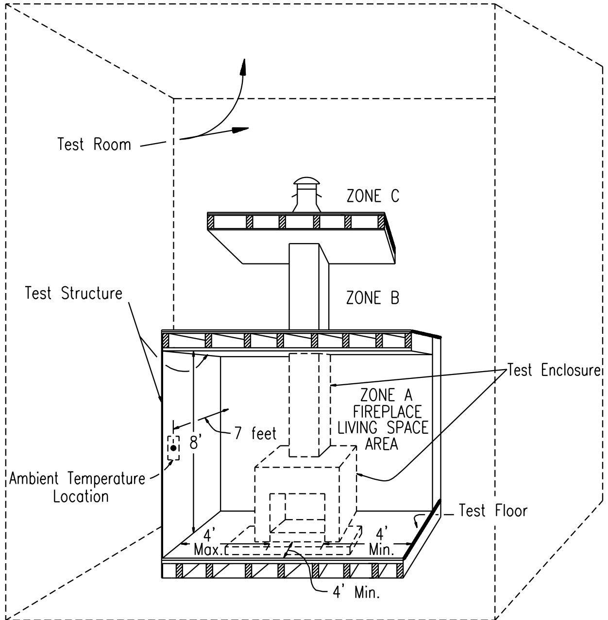
Figure 9.1 Typical test structure within test room
