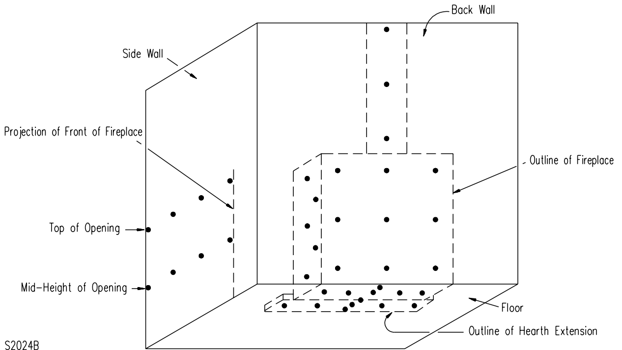
Figure 10.3 Typical thermocouple locations (-) Back, side, and floor at fireplace (Zone A)
