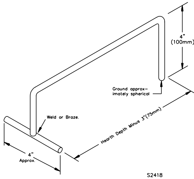
Figure 13.1 Andiron
