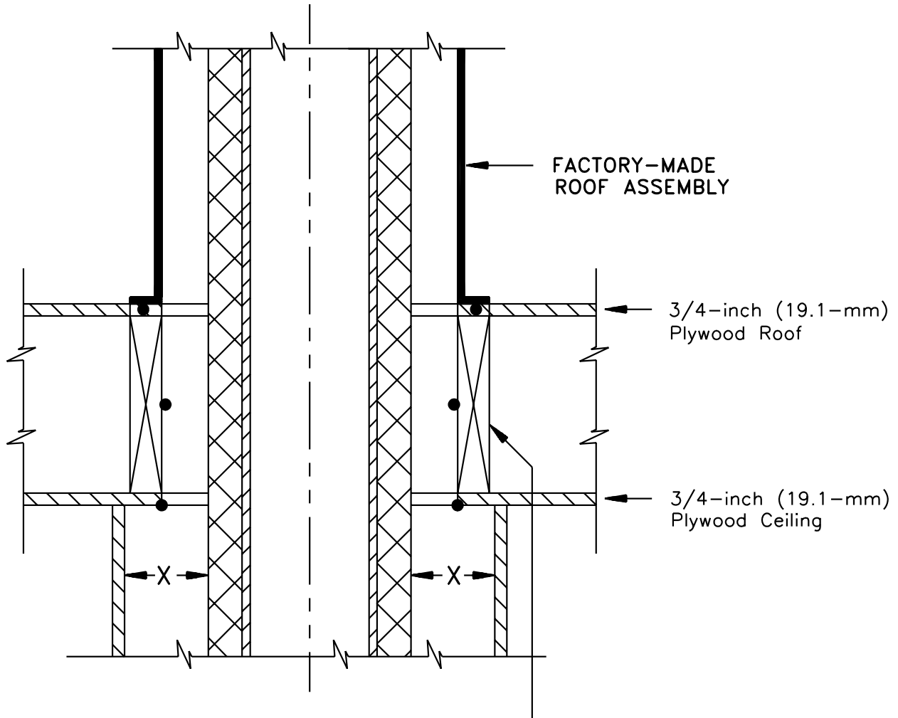
Figure 9.9 Test structure details for roof assembly (Roof assembly smaller than enclosure area)
