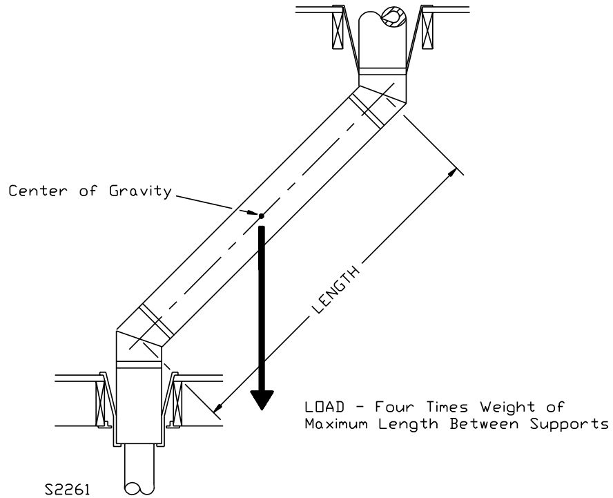
Figure 17.2 Load test for chimney elbows
