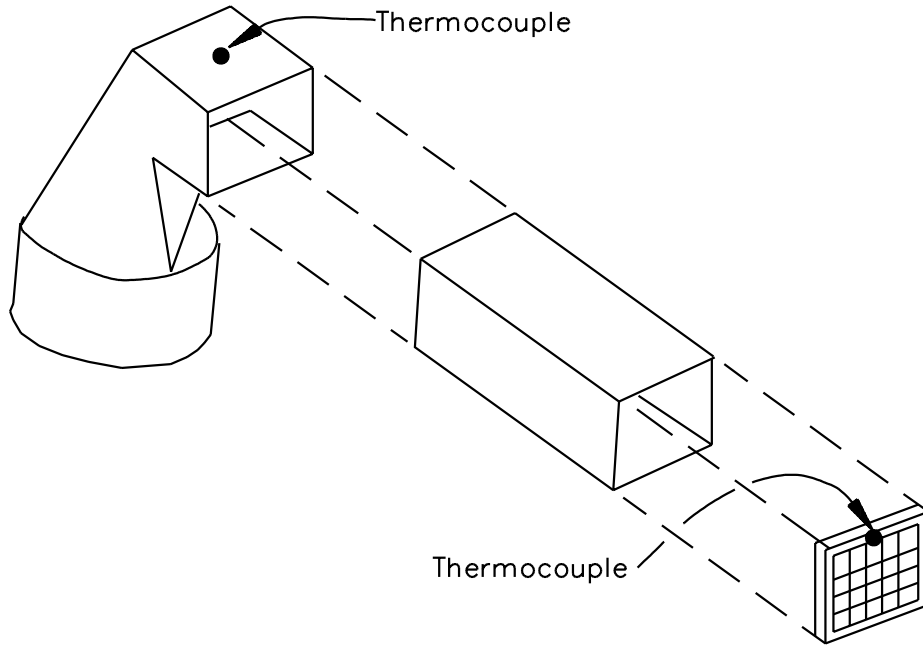
Figure 10.9 Typical thermocouple locations (Air duct fittings)
