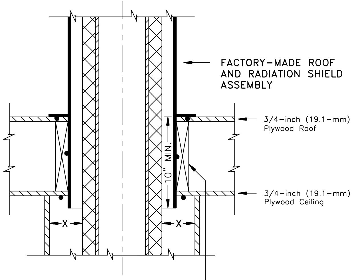
Figure 9.10 Test structure details for roof assembly (Roof assembly of type not requiring field alteration to conform to roof line)
