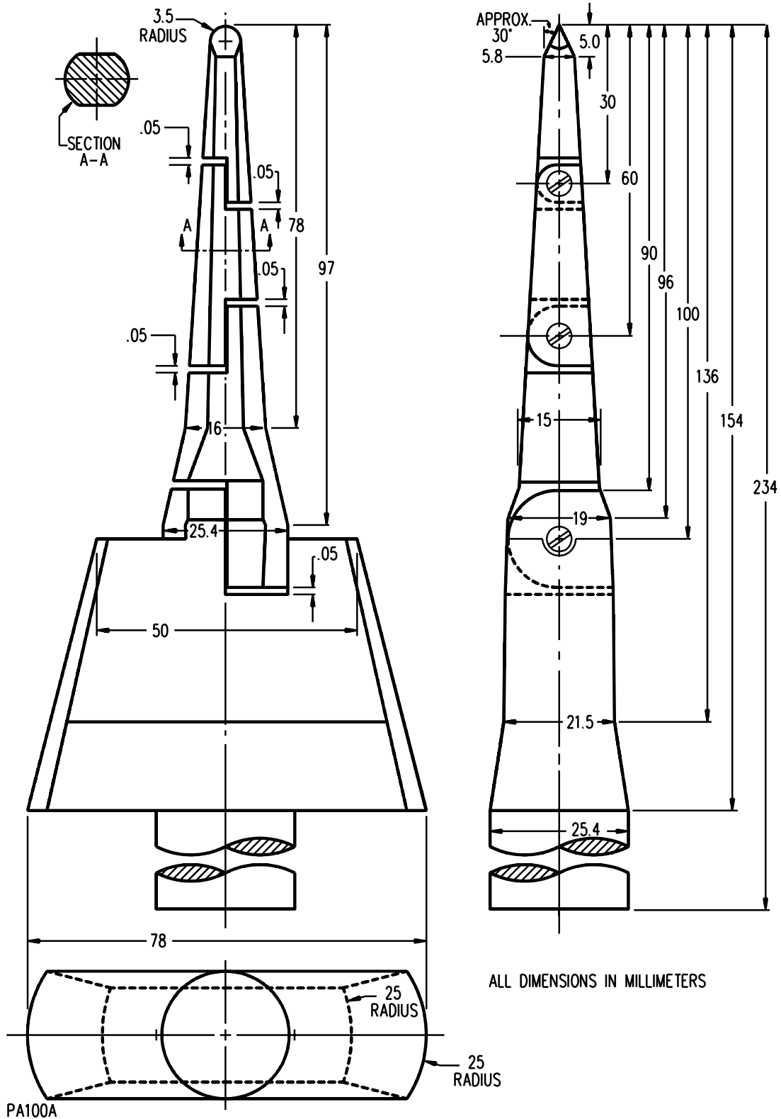
Figure 28.1 Accessibility probe
