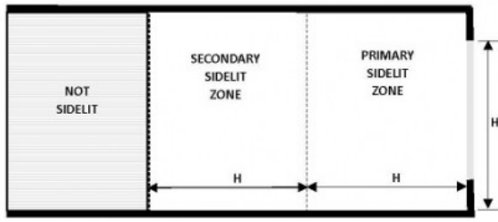
(a) Section View of Primary Sidelit Zone and Secondary Sidelit Zone
