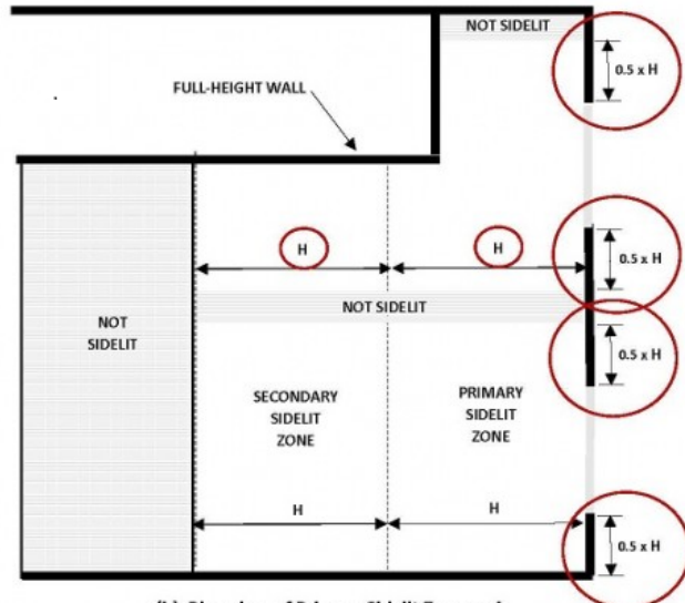
(b) Plan view of Primary Sidelit Zone and Secondary Sidelit Zone
