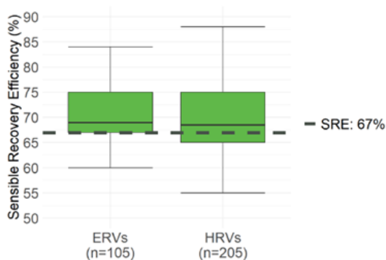
Figure 1: Boxplot of SRE of ERVs and HRVs (30-100cfm) from the HVI Certified Products database (Source: TRC 2020 pdf p. 86)
