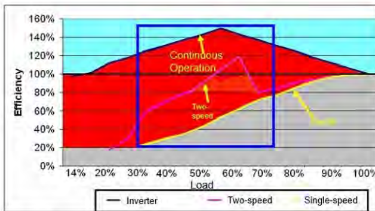
Figure 1: HVAC Equipment Efficiency at Various Part-Loads
