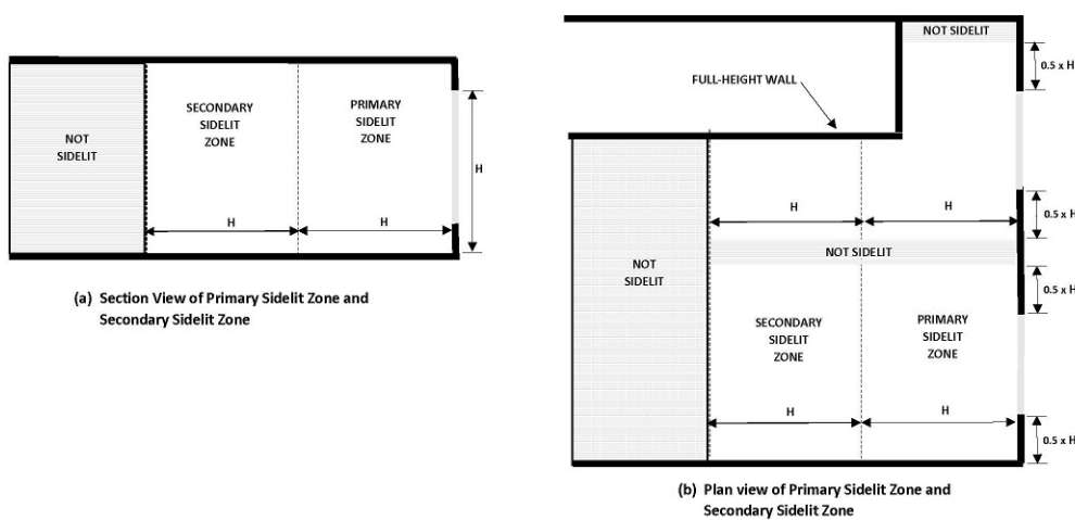
FIGURE C405.2.4.2(2) DAYLIGHT ZONE UNDER A ROOFTOP MONITOR
