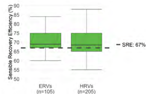
Figure 1: Boxplot of SRE of ERVs and HRVs (30-100cfm) from the HVI Certified Products database (Source: TRC 2020 pdf p. 86)
