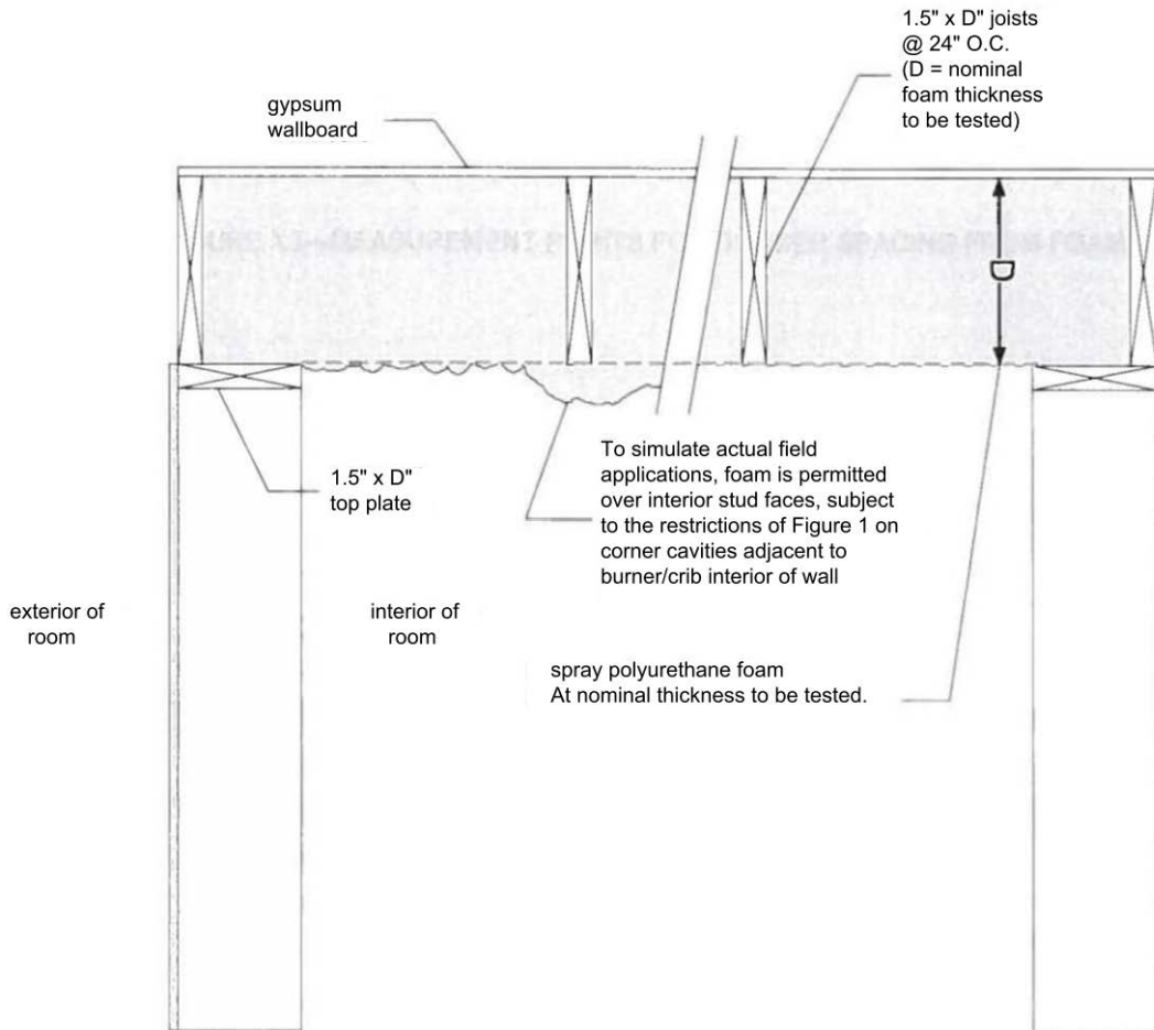
FIGURE 3—SIDE VIEW OF CEILING CONSTRUCTION
