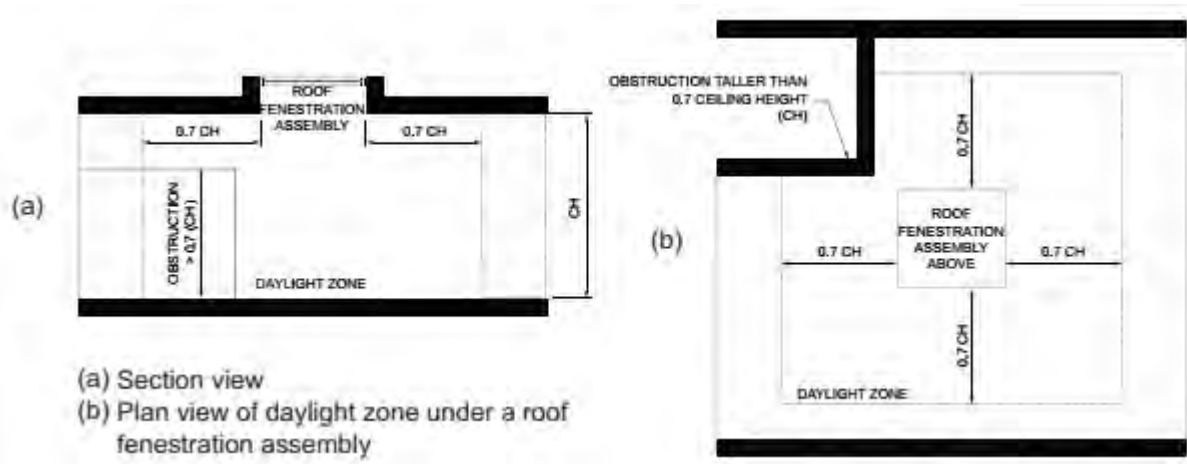
FIGURE C405.2.4.3 TOPLIT DAYLIGHT ZONE
