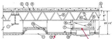
Ceiling Membrane Ceiling Damper
