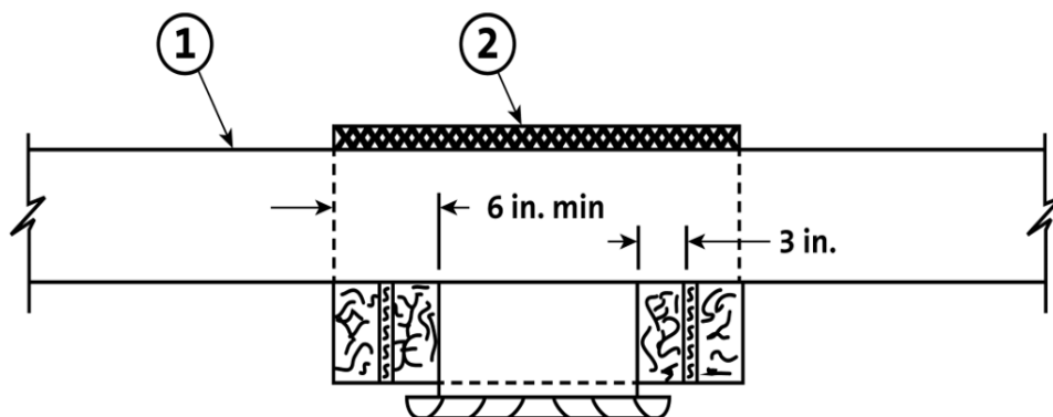
Longitudinal Cross-Section
