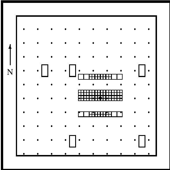
FIGURE 3: Layout of Plastic Test P-1.
