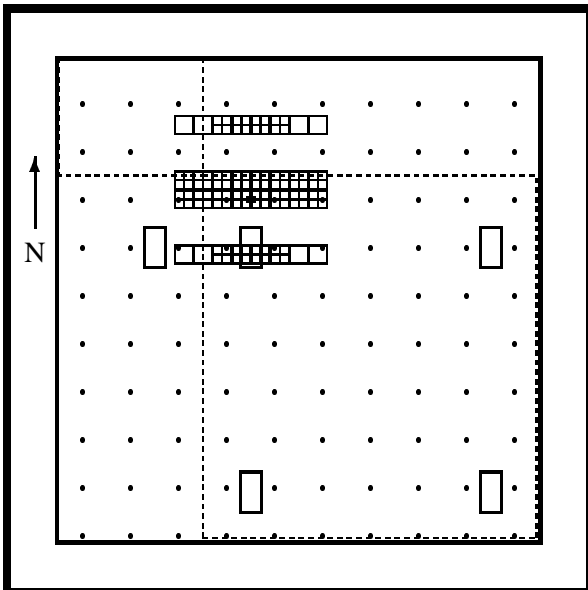
FIGURE 5: Layout of Plastic Test P-3.
