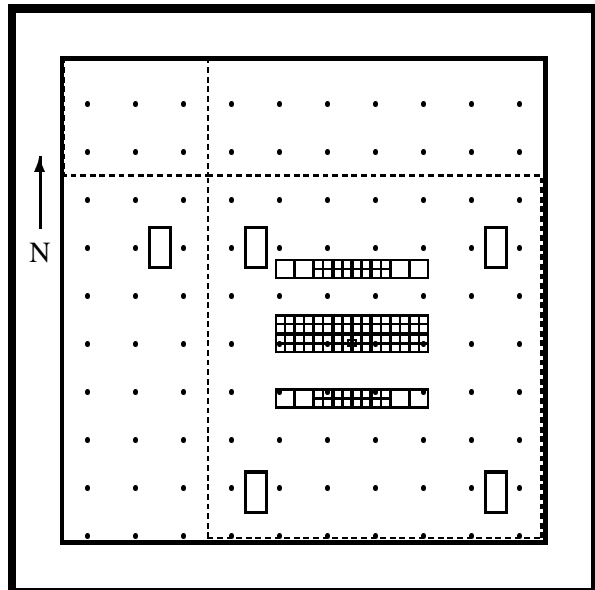
FIGURE 6: Layout of Plastic Tests P-4 and P-5.
