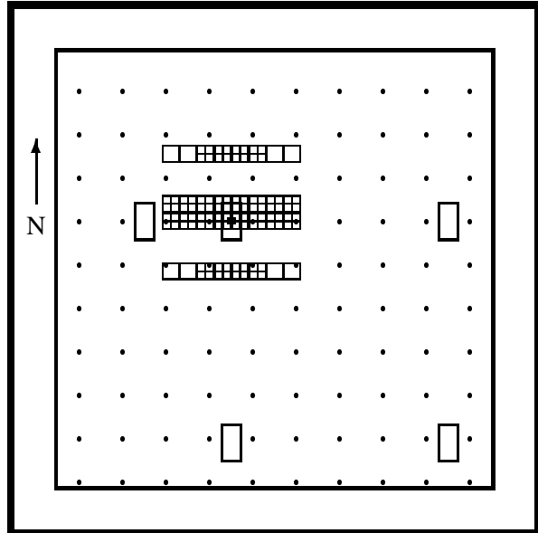
FIGURE 4: Layout of Plastic Test P-2.
